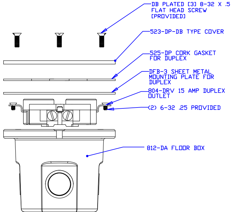
RIGHT [EXPLODED]
