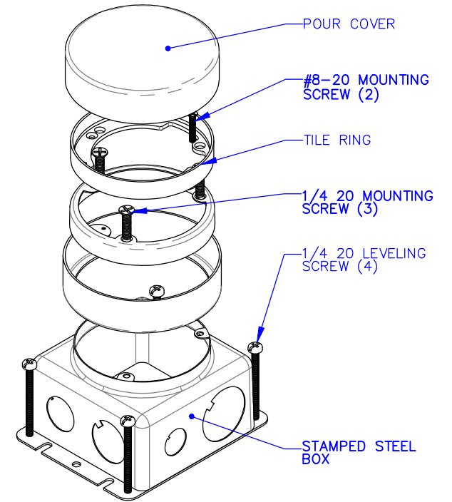
ISOMETRIC (EXPLODED)
