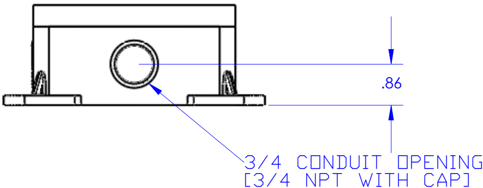
RIGHT VIEW
