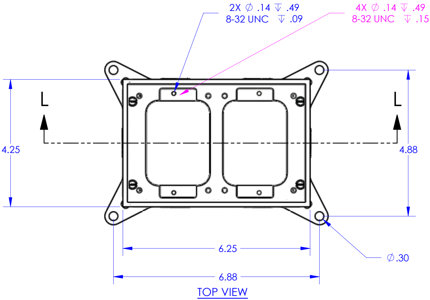
TOP VIEW
