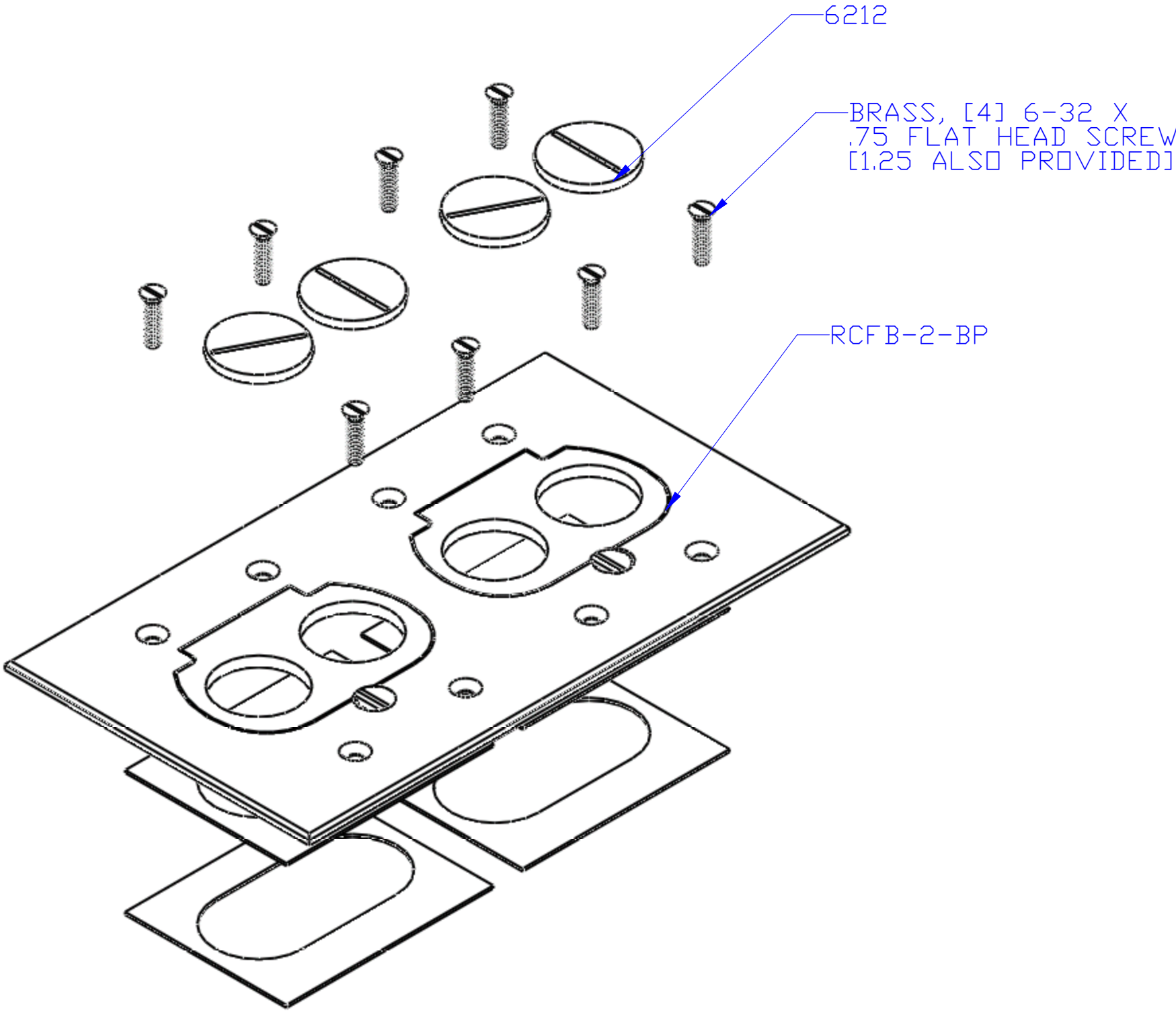
ISOMETRIC (EXPLODED) VIEW
