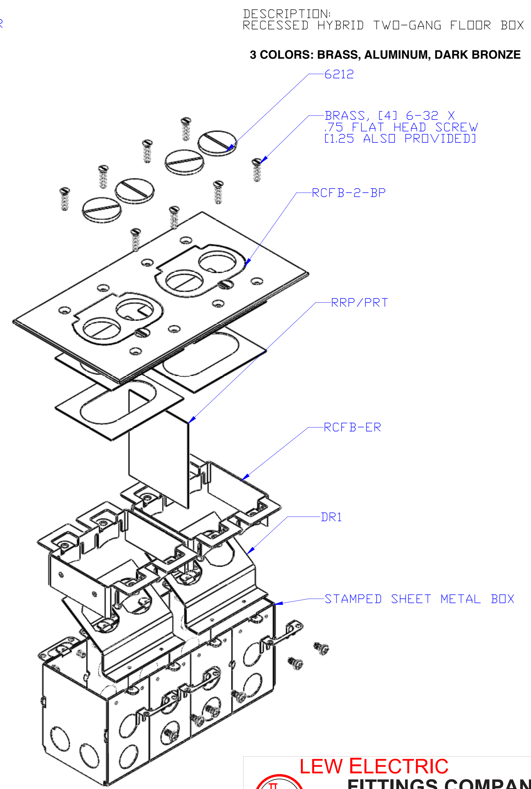
ISOMETRIC (EXPLODED) VIEW
