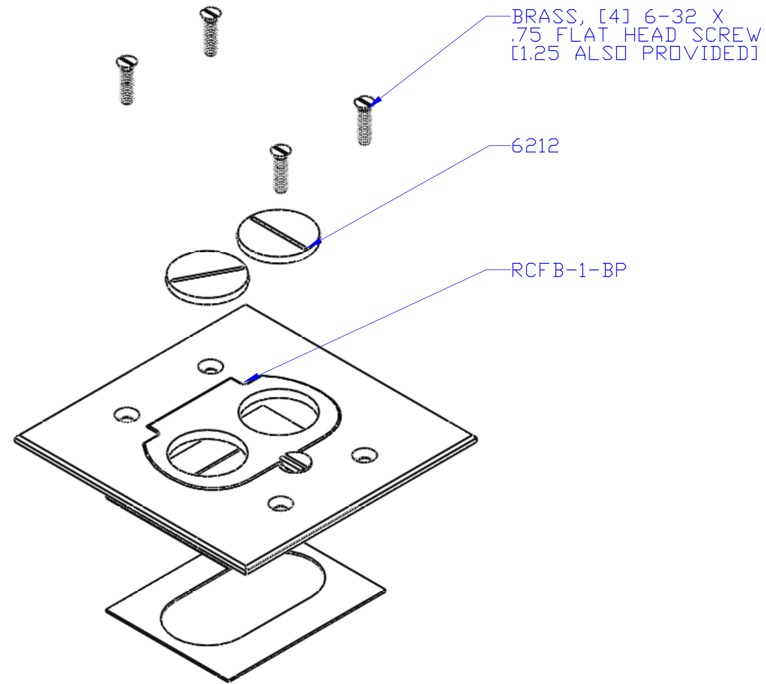
ISOMETRIC (EXPLODED) VIEW
